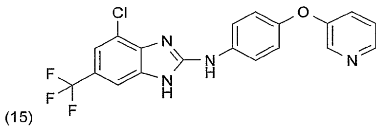
(4-Chlor-6-trifluormethyl-1H-benzimidazol-2-yl)-[4-(pyridin-3-yloxy)-phenyl]-amin
